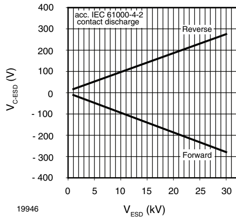
Figure 9. Typical Clamping Voltage at \pm ESD Contact Discharge (acc. IEC 61000-4-2)
